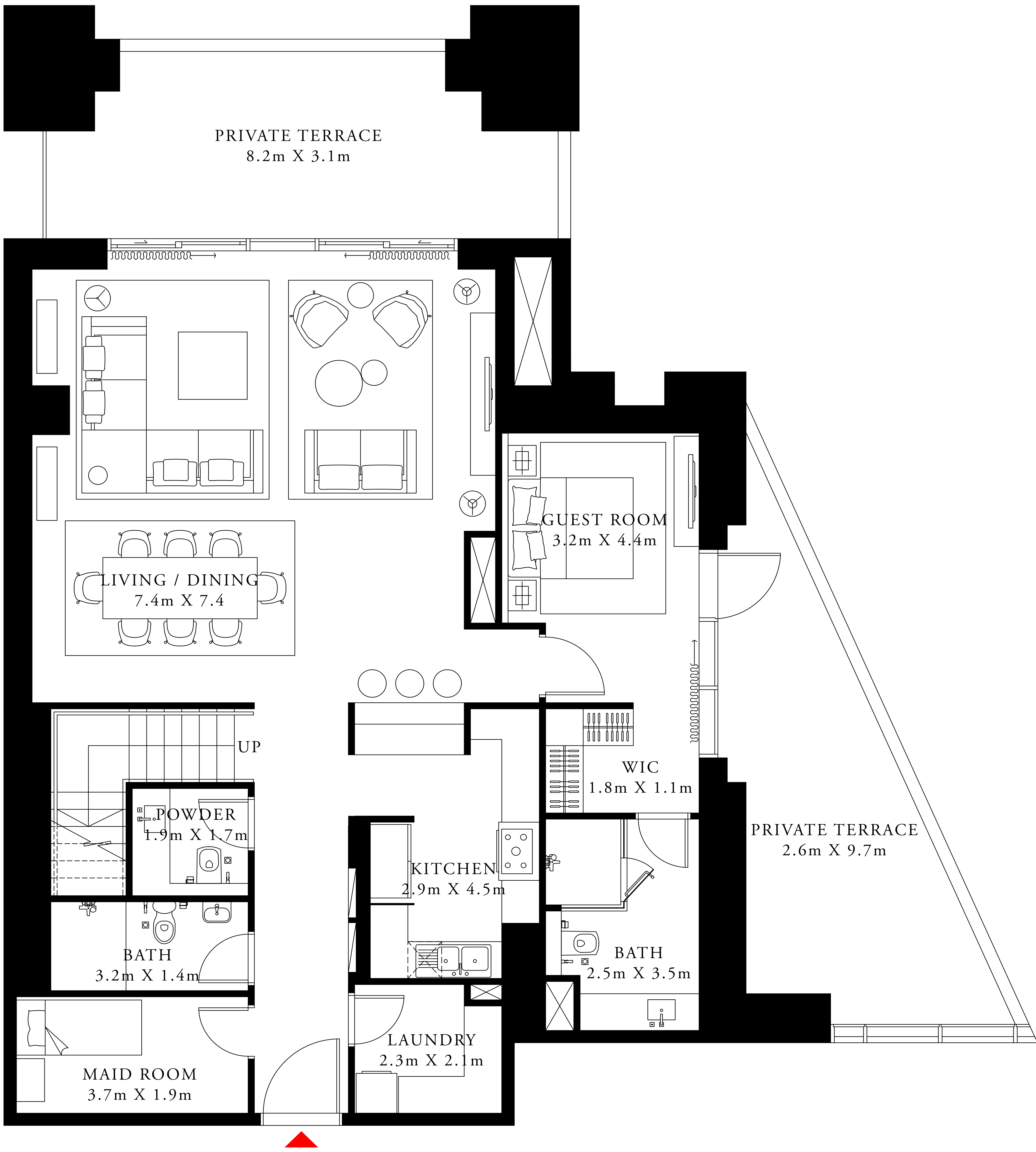
LOWER LEVEL
